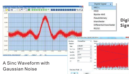
Gaussian Noise
