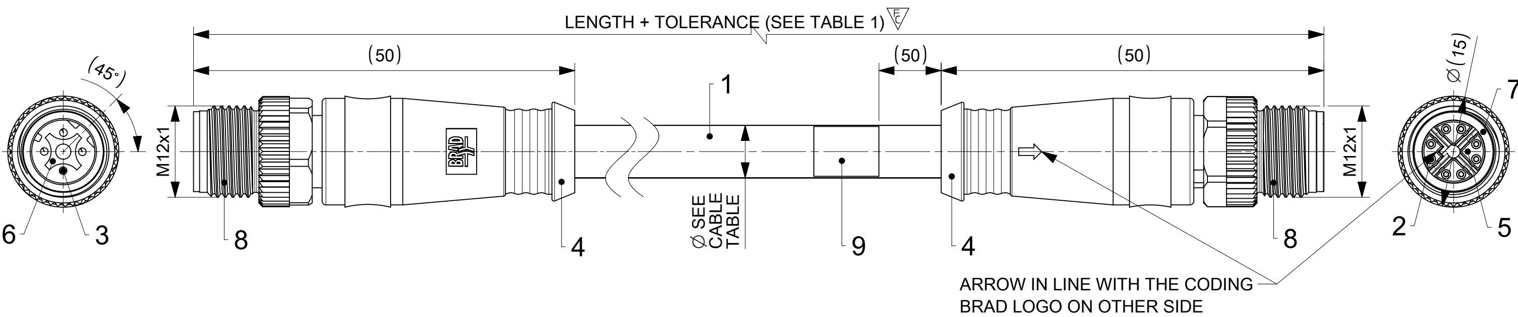
M12 4P DC MALE FRONT VIEW ACCORDING IEC 61076-2-101
