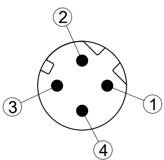
M12 4P DC MALE FRONT VIEW ACCORDING IEC 61076-2-101
