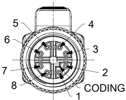
M12 X-CODE MALE FRONT VIEW
