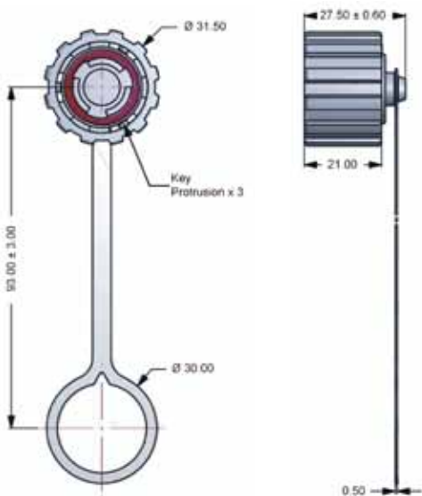
Plastic design / Bayonet locking
