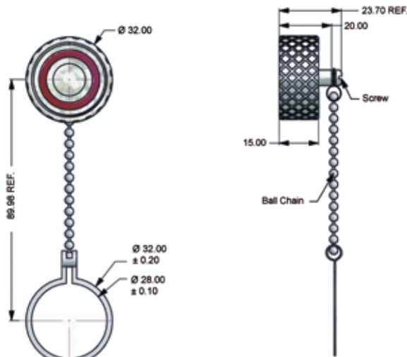
Metal design / M28 thread
