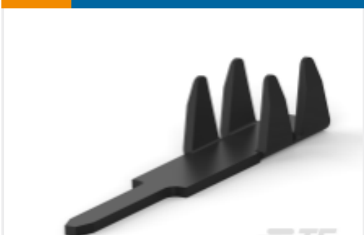
TE Part # 1-86557-9 2.54mm FFC Connectors Pin Contacts
