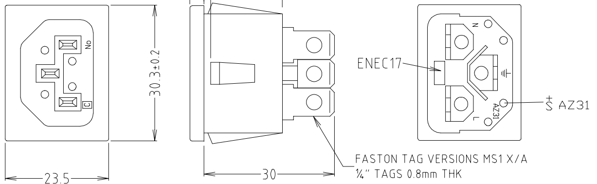
CL19193 - MS1X 3 pole Mains inlet
