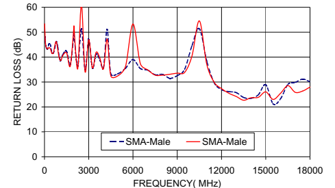
086-8SM+ RETURN LOSS
