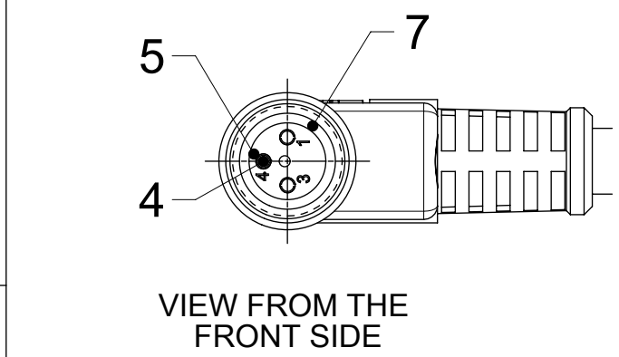
CONTACTS POSITION FRONT VIEW:
