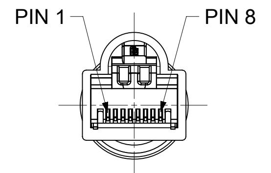
VIEW FROM FRONT SIDE RJ45 MALE
