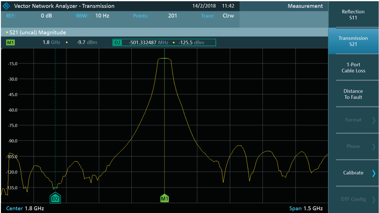
R&S®FPC1500 S_{21} scalar transmission measurement with the R&S®FPC-K42 option
