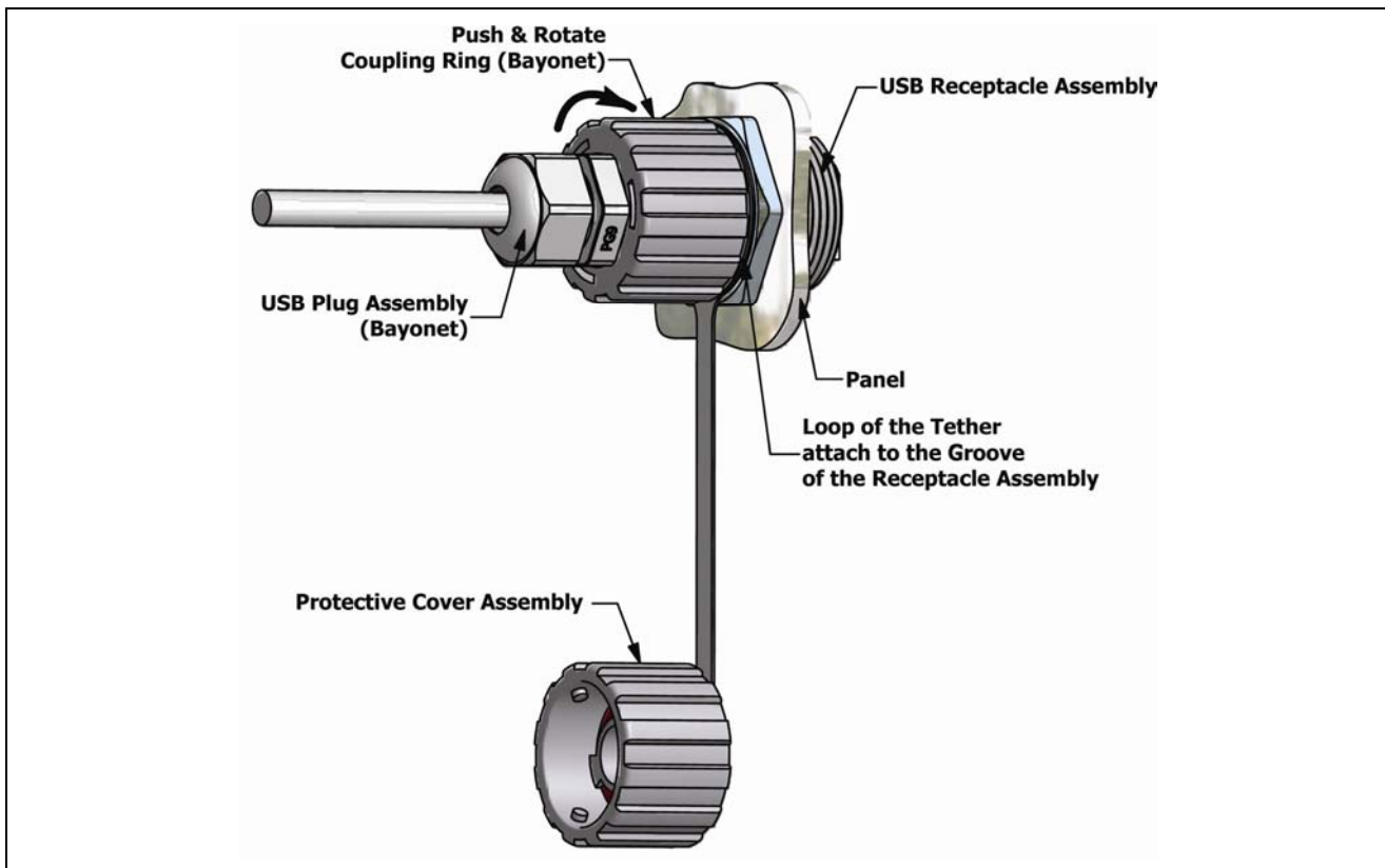
Figure 9-1: USB Plug and Receptacle Engagement (Bayonet Locking Style)
