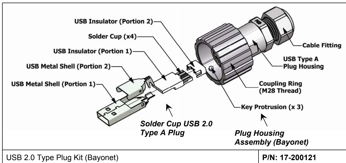
Figure 1-1: The USB 2.0 Type A Plug Kit
