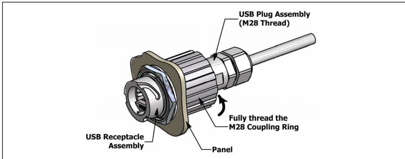
Figure 9-2: USB Plug and Receptacle Engagement (M28 Thread)
