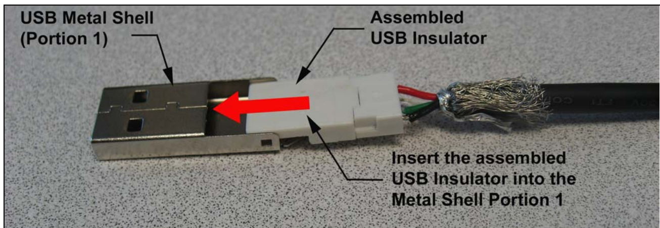
Figure 3-6: Assembly of the USB Insulator and Metal Shell Portion 1
