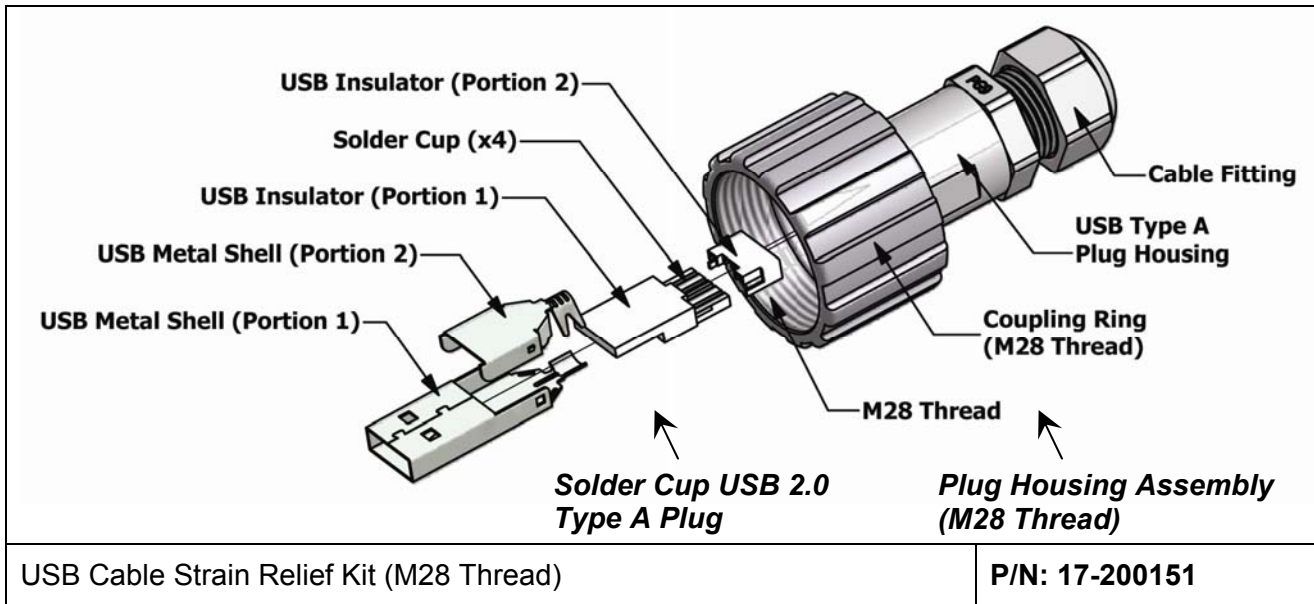
Figure 2-1: USB Cable Strain Relief Kit
