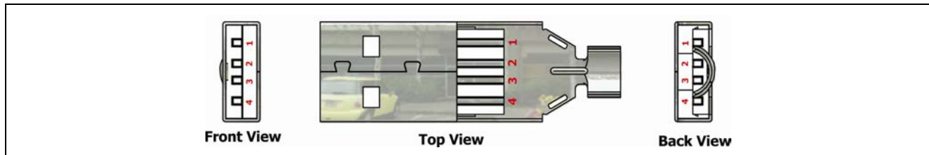
Figure 3-1: Pin Number Assignment for USB Type A Plug
