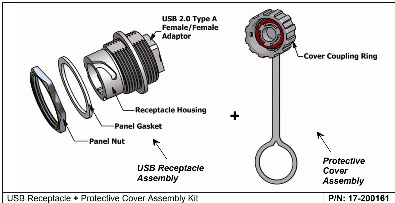
Figure 7-1: USB Receptacle + Protective Cover Assembly Kit
