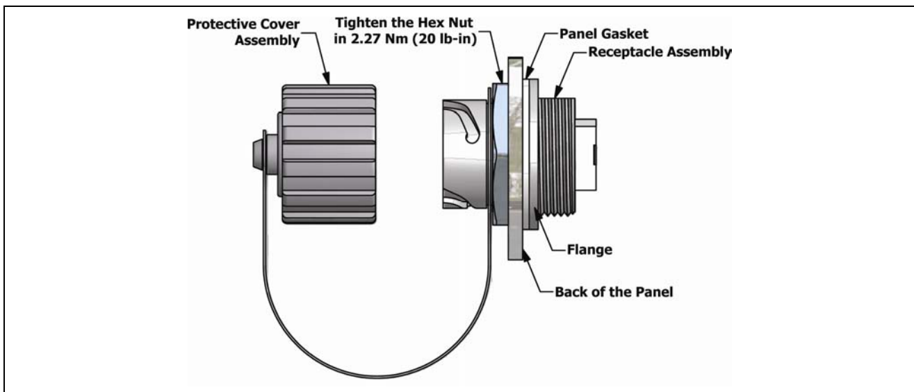
Figure 8-2: The Receptacle Panel Front Mounting
