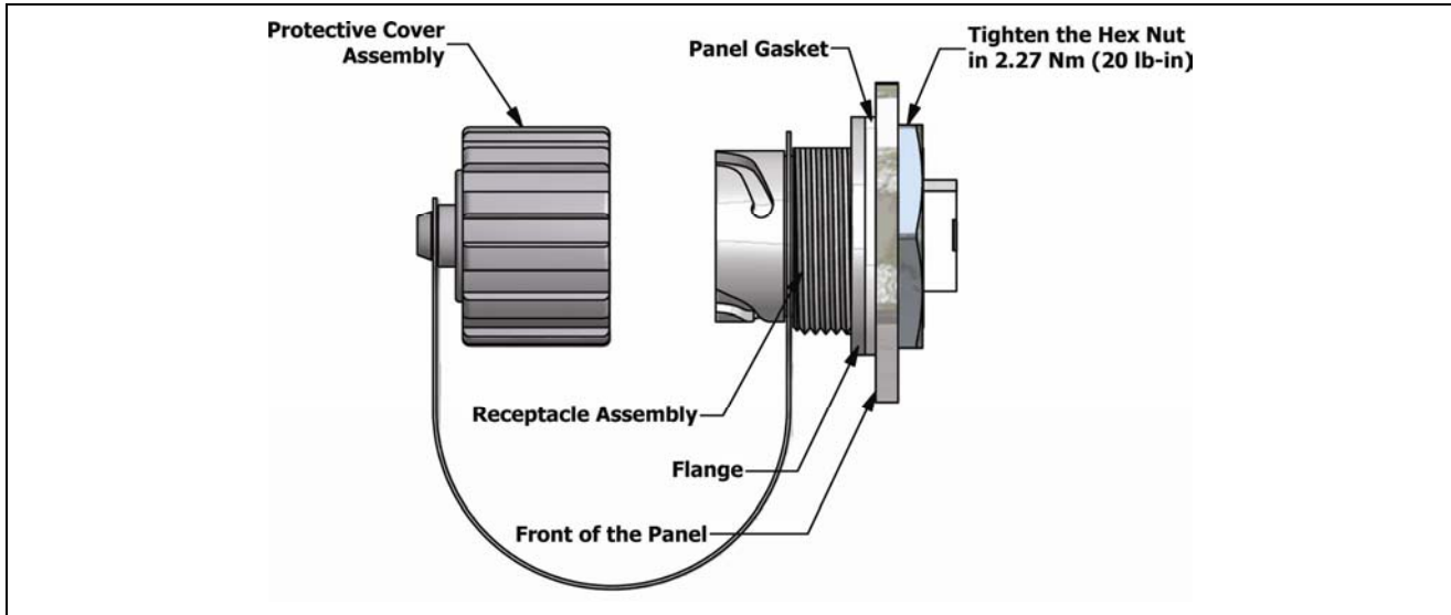
Figure 8-3: The Receptacle Panel Rear Mounting
