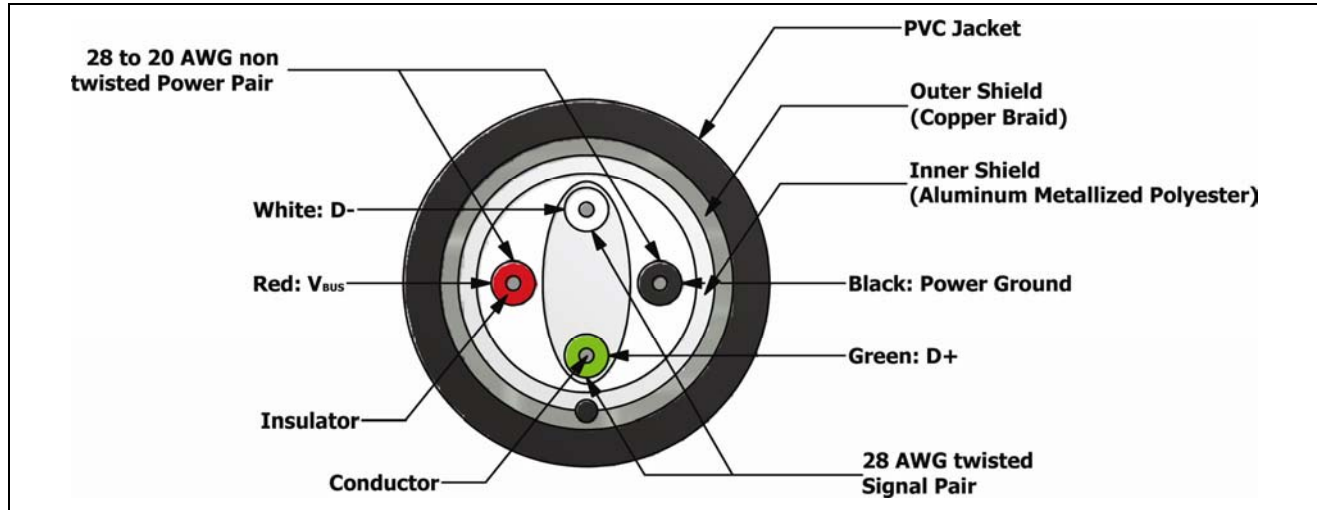
Figure 3-2: High Speed USB Cable Construction
