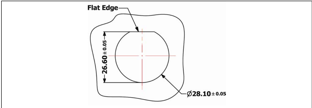
Figure 8-1: Recommended Panel Cutout
