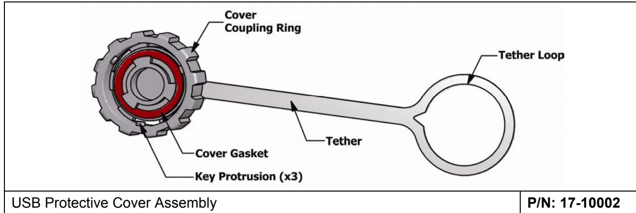
Figure 6-1: Protective Cover Assembly
