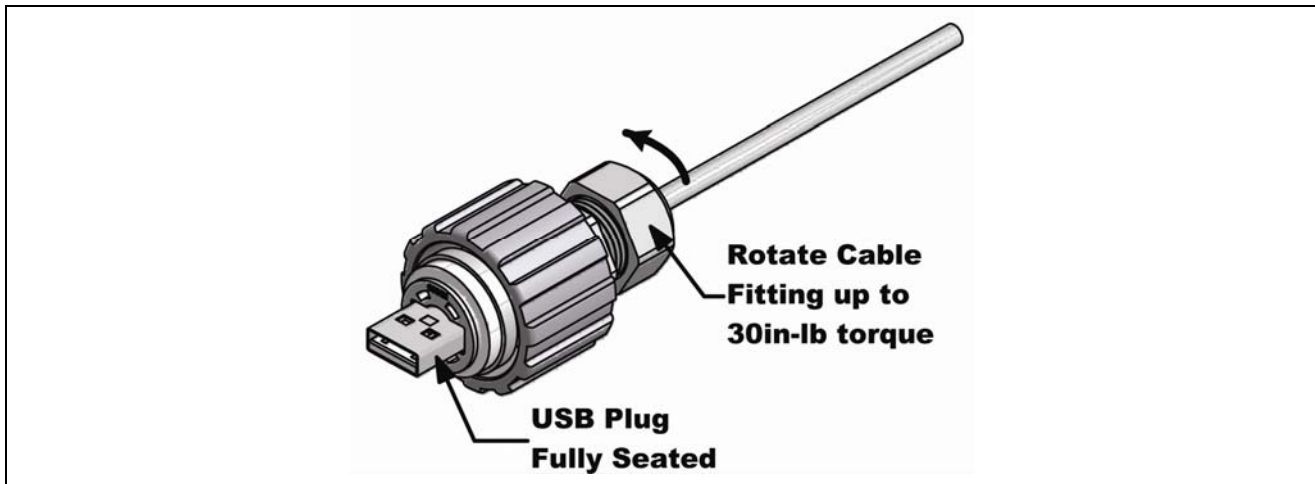
Figure 4-2: Assembly of the USB Type A Plug Housing (Step 2)
