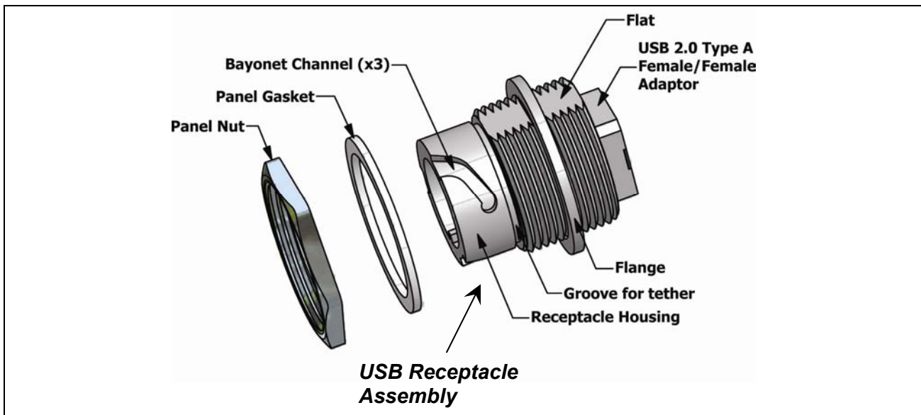
Figure 5-1: USB 2.0 Receptacle Assembly Kit
