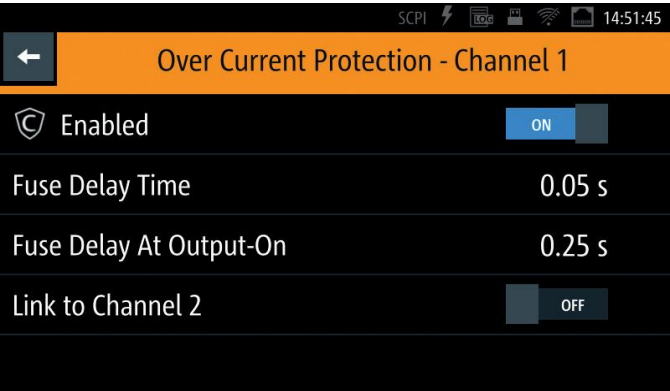
Electronic fuse with additional functions: “Fuse delay at output-on” specifies how long the fuse remains inactive after the channel is activated. The sensitivity of the fuse is specified using the “Fuse delay time”.
