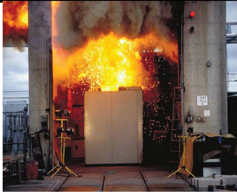
Figure 1. Demonstration of the power of an Arc Flash (ewb engineering http://www.ewbengineering.com/ )
