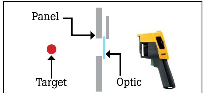
Figure 10. An example of negative error. Target Temperature = 50 °C Ambient Temperature = 30 °C Window Optic Temperature = 30 °C Indicated Temperature = 45 °C
