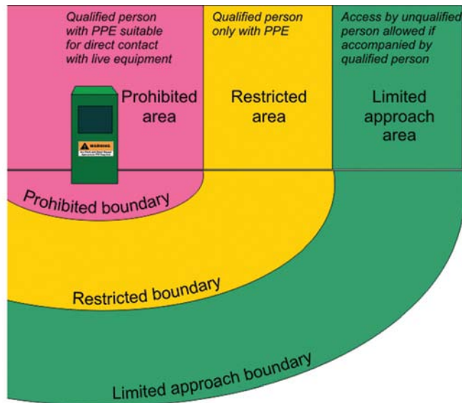
Figure 2. The shock hazard boundaries
