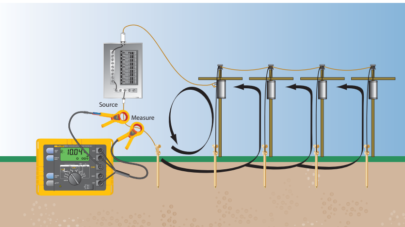
Test current paths in the stakeless method.
