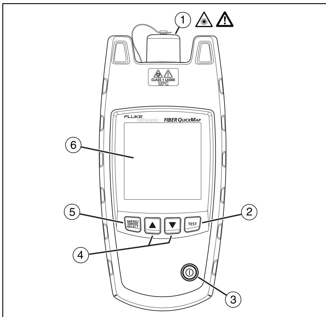
Figure 2. Physical Features
