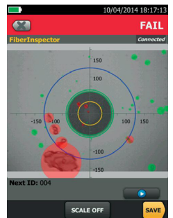
FiberInspector probe
