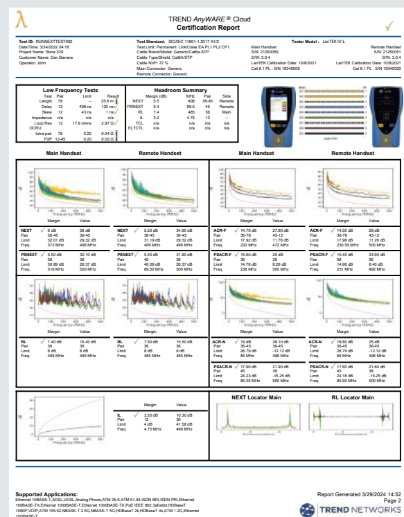
TREND AnyWARE Cloud Test Report
