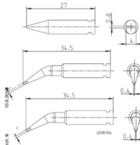
XH D Soldering tip 4,0x0,8mm T0054491199
