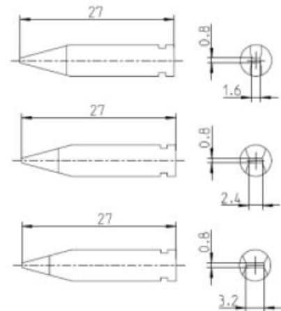
XH C Soldering tip 3,2x0,8mm T0054491099
