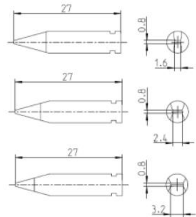
XH C Soldering tip 3,2x0,8mm T0054491099
