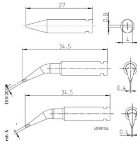
XH D Soldering tip 4,0x0,8mm T0054491199
