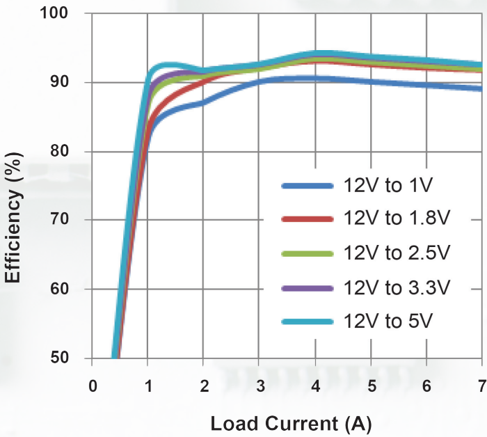
Efficiency vs. Load Current
