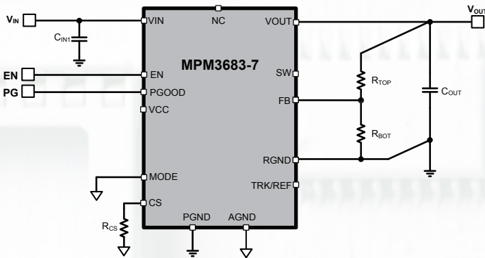
Typical Application
