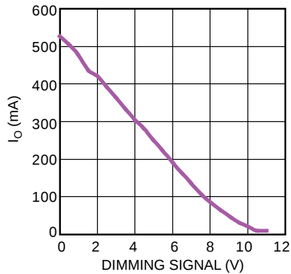
Analog Dimming Curve @ 110 Vac
