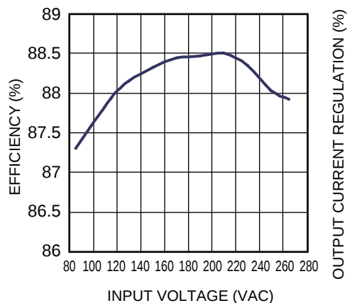
Efficiency
