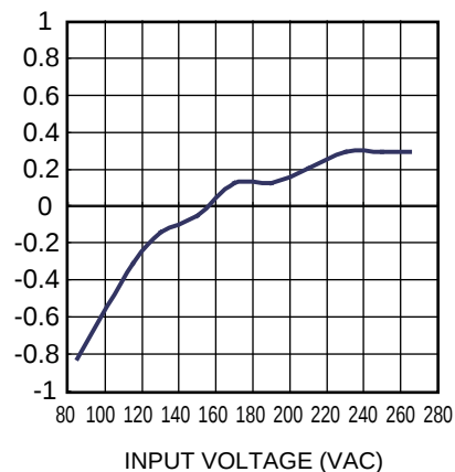
Output Current Regulation
