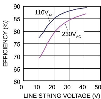
Efficiency vs. String Voltage
