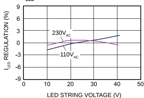
I_{LED} Regulation vs. String Voltage
