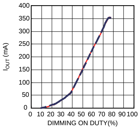
Dimming Curve
