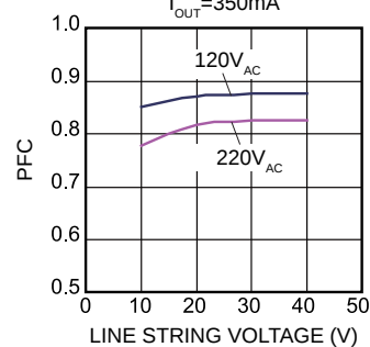
Passive PFC
