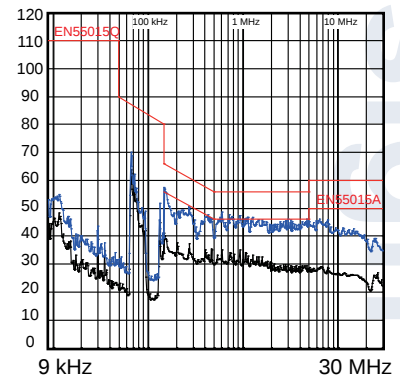
Conducted EMI
