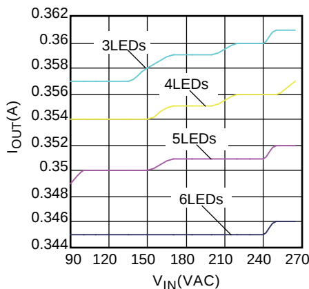
Line/Load Regulation
