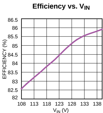
Efficiency vs VIN
