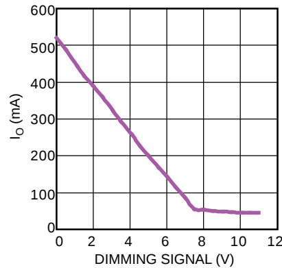
Analog Dimming Curve @ 220 Vac
