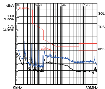
Conducted EMI 230V AC /50Hz, Line Wire
