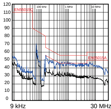
Conducted EMI
