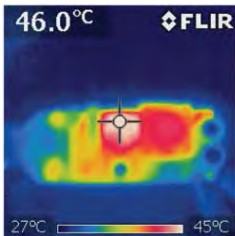
Without Dimmer
