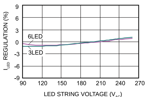
I_{LED} Regulation vs. Input Voltage
