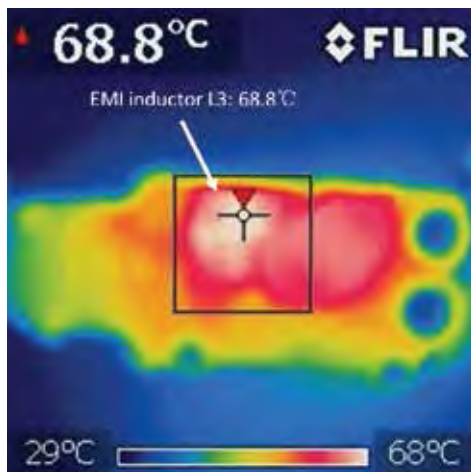
Without Dimmer
