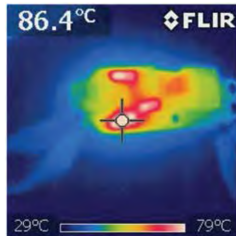
With Dimmer at 90% Dimming on Phase
